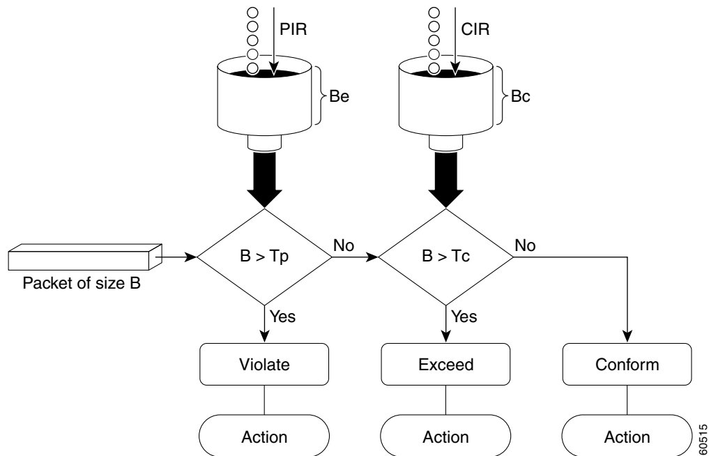
Figure 1-1 Marking Packets and Assigning Actions with the Two-Rate Policer
