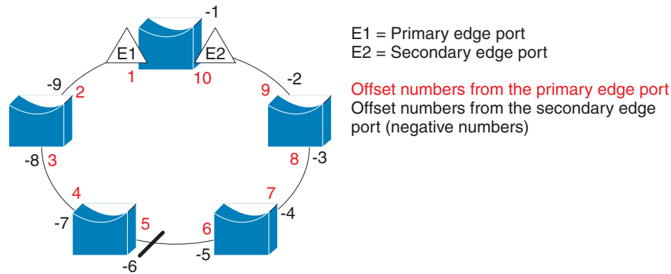
Figure 1-2 Neighbor Offset Numbers in a REP Segment
