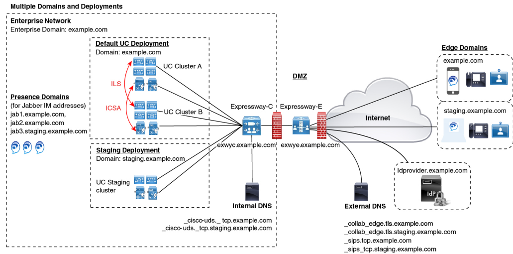
Figure 26: Multiple Domains with Separate Deployments
