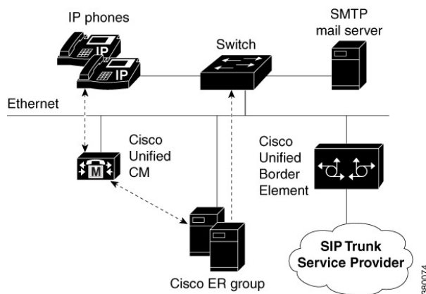
Figure 3: Cisco Emergency Responder and a SIP Trunk Service Provider
