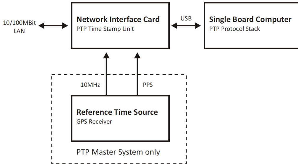
Figure 44 M600 Block Diagram
