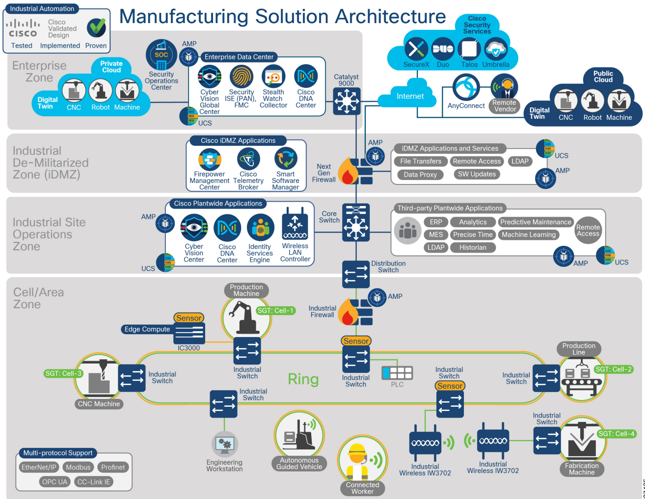
Figure 2 Manufacturing Solution Architecture
