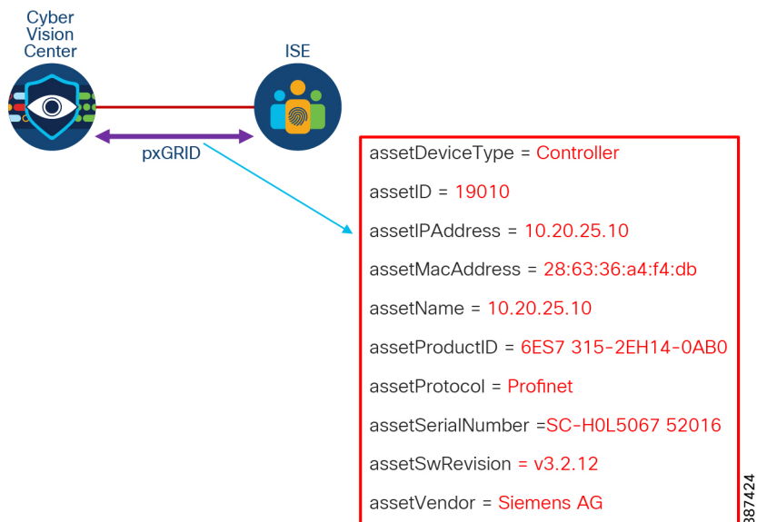
Figure 5 Cisco Cyber Vision Exporting Attributes to ISE
