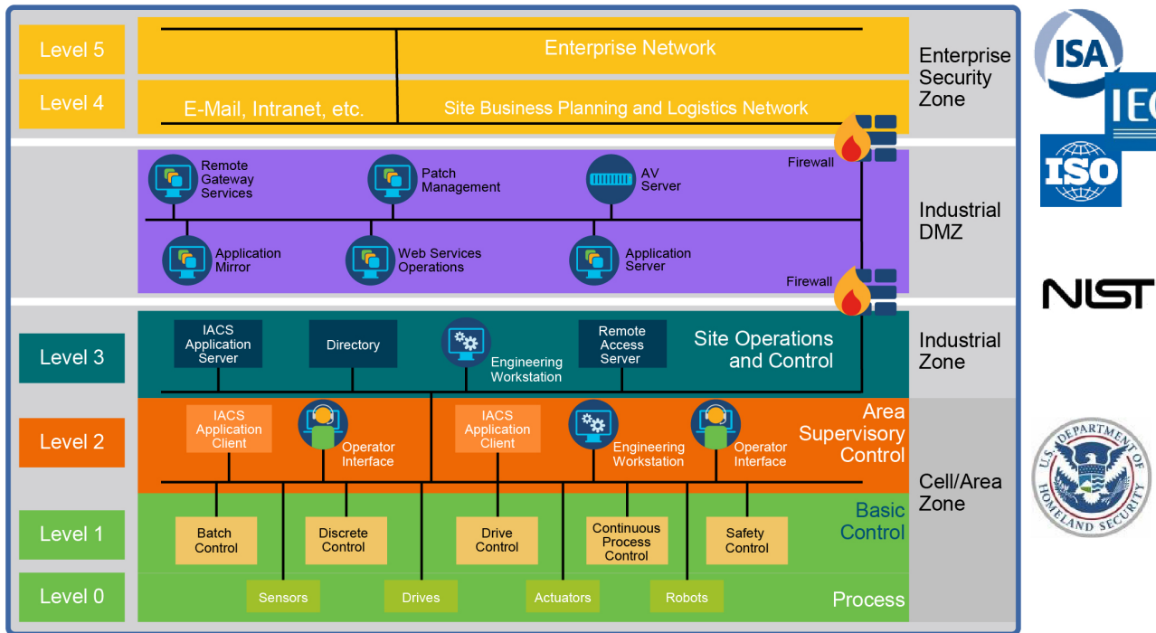
Figure 1 Industrial Plant Reference Architecture with IDMZ
