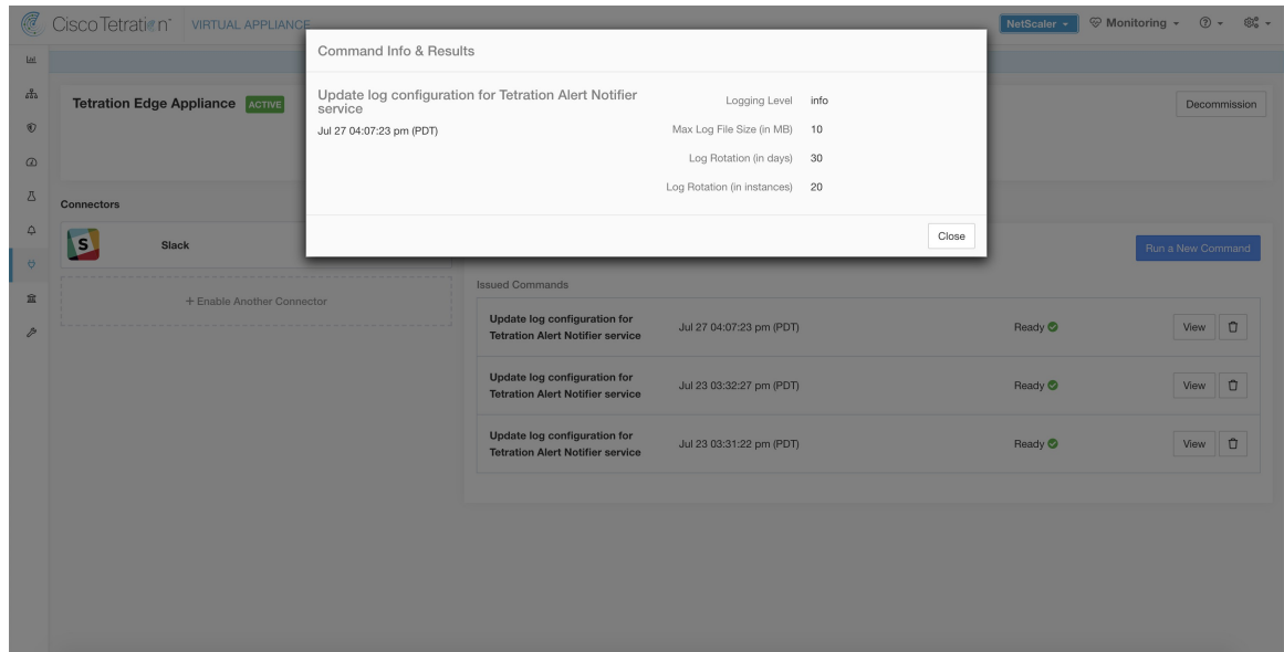
Figure 150: Update the log configuration on Secure Workload Alert Notifier Docker service in Secure Workload Edge appliance
