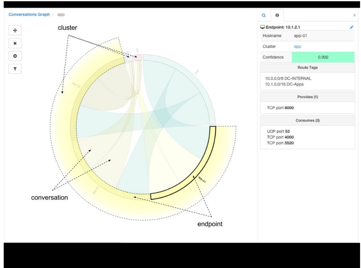
Figure 328: Conversations Chart View
