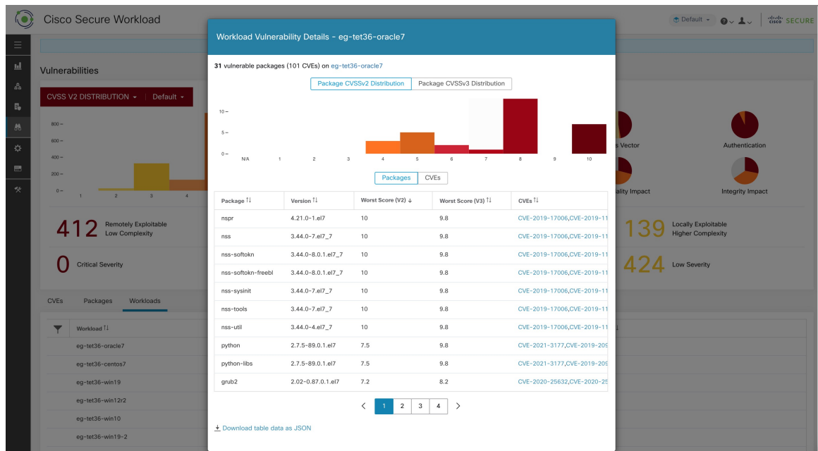
Figure 515: Vulnerability Details in an Impacted Workload
