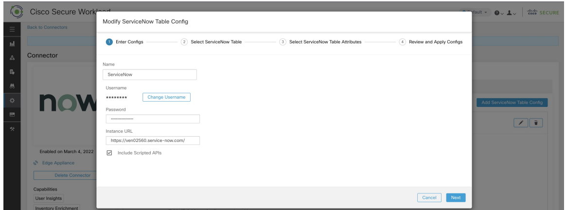
Figure 69: Secure Workload Fetches the Table Info from ServiceNow Instance
