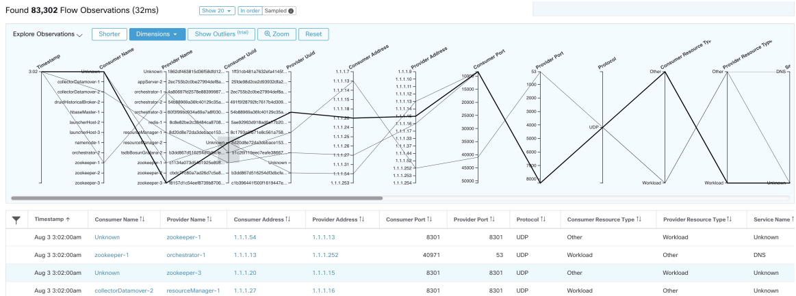
Figure 374: Explore with selection
