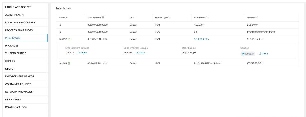
Figure 219: Workload Interface List
