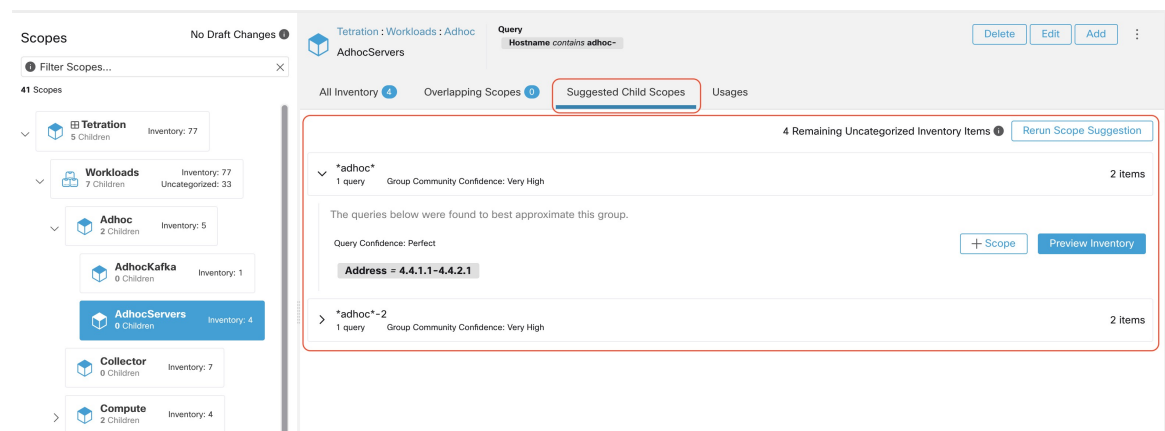
Figure 201: Scope Suggestion Output Queries
