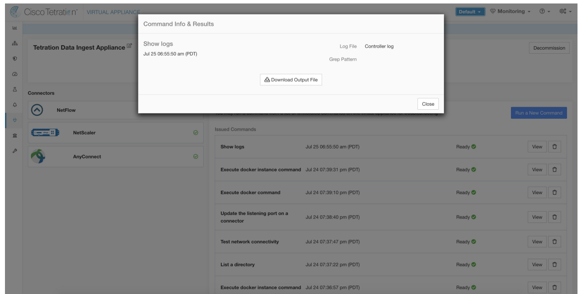
Figure 136: Download Show Logs output from Secure Workload Ingest appliance
