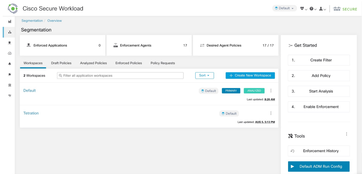
Figure 283: Policy automatically getting rejected by Auto-pilot rule
