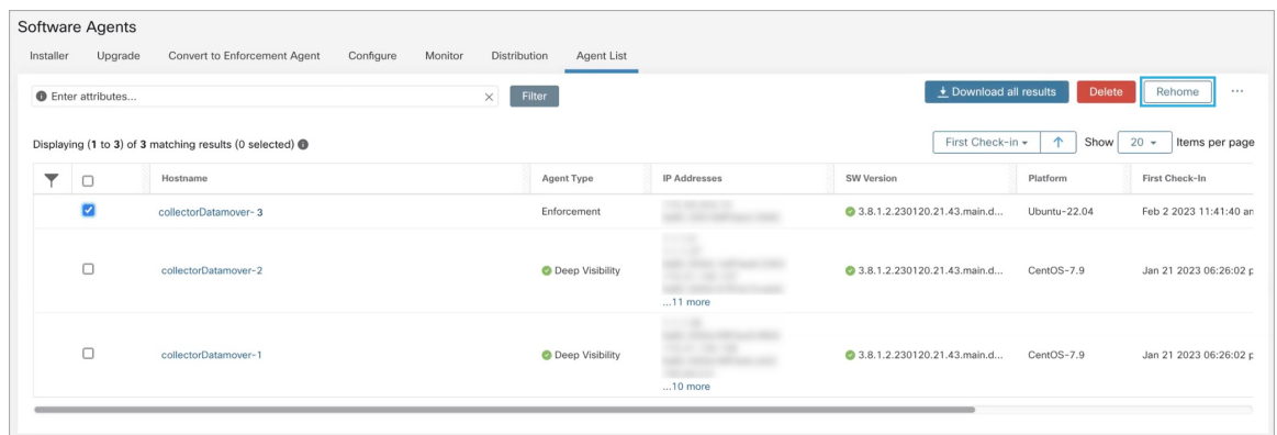
Figure 18: Enable Agent Rehoming
