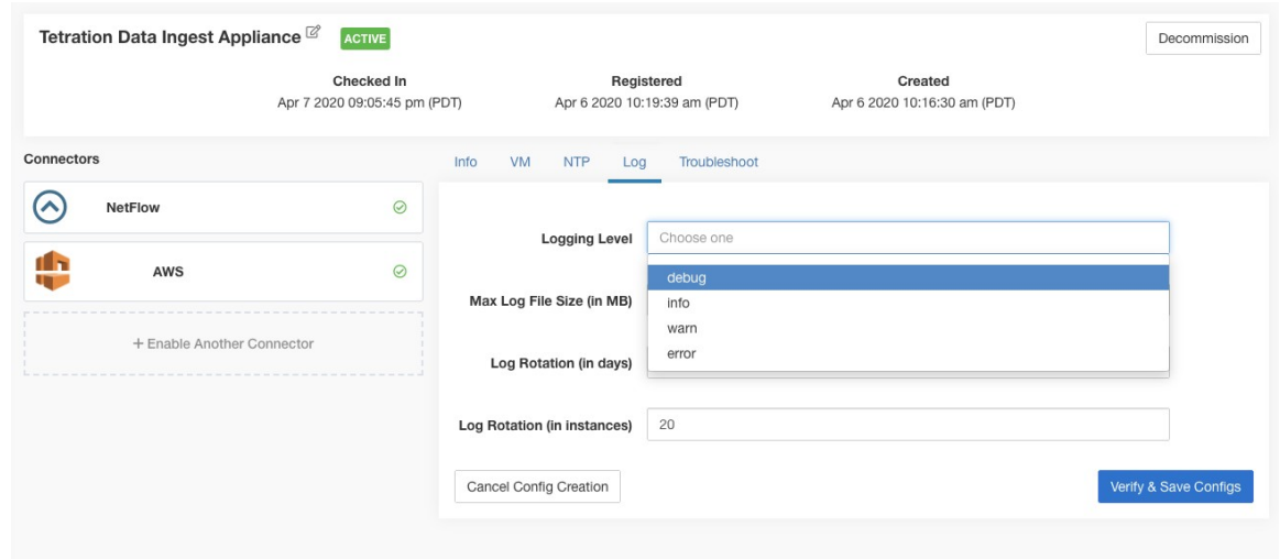
Figure 127: Log configuration on the appliance
