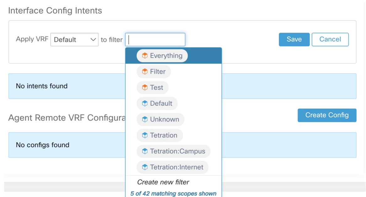
Figure 14: Interface Configuration Intents
