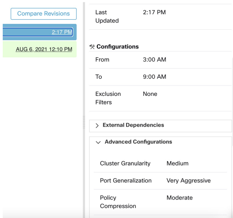
Figure 260: Configurations used for particular automatic policy discovery runs
