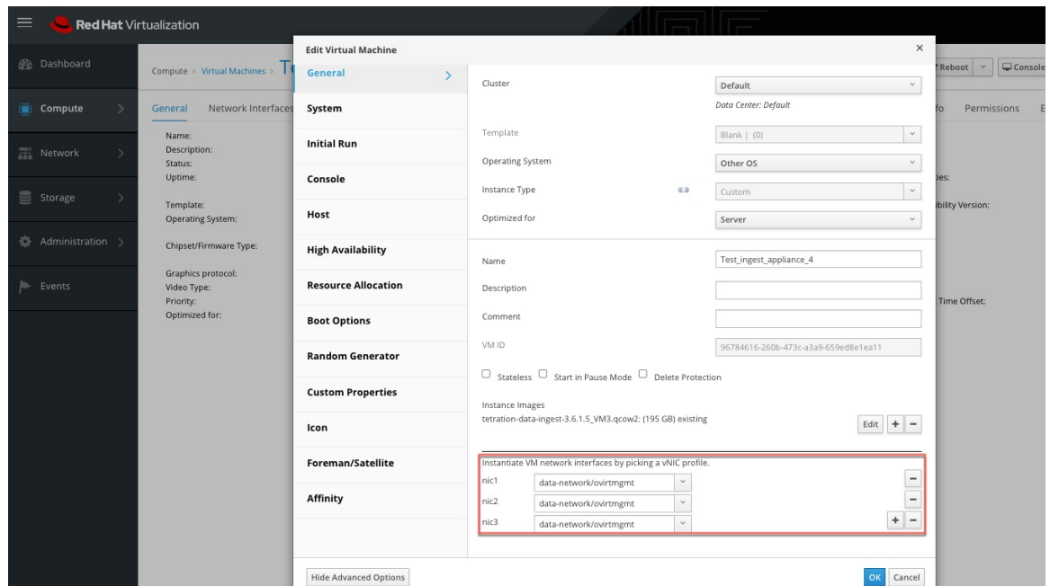
Figure 116: Example of Configuring Network Interfaces in KVM-Based Environments
