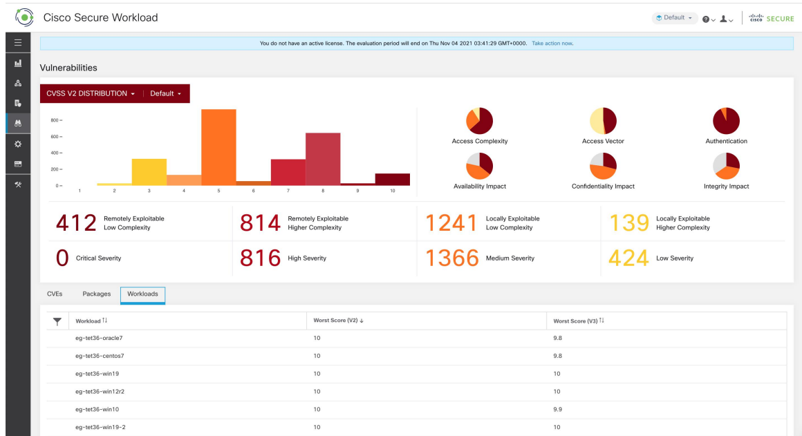
Figure 514: Workloads Tab Listing Vulnerable Workloads in Specified Scope
