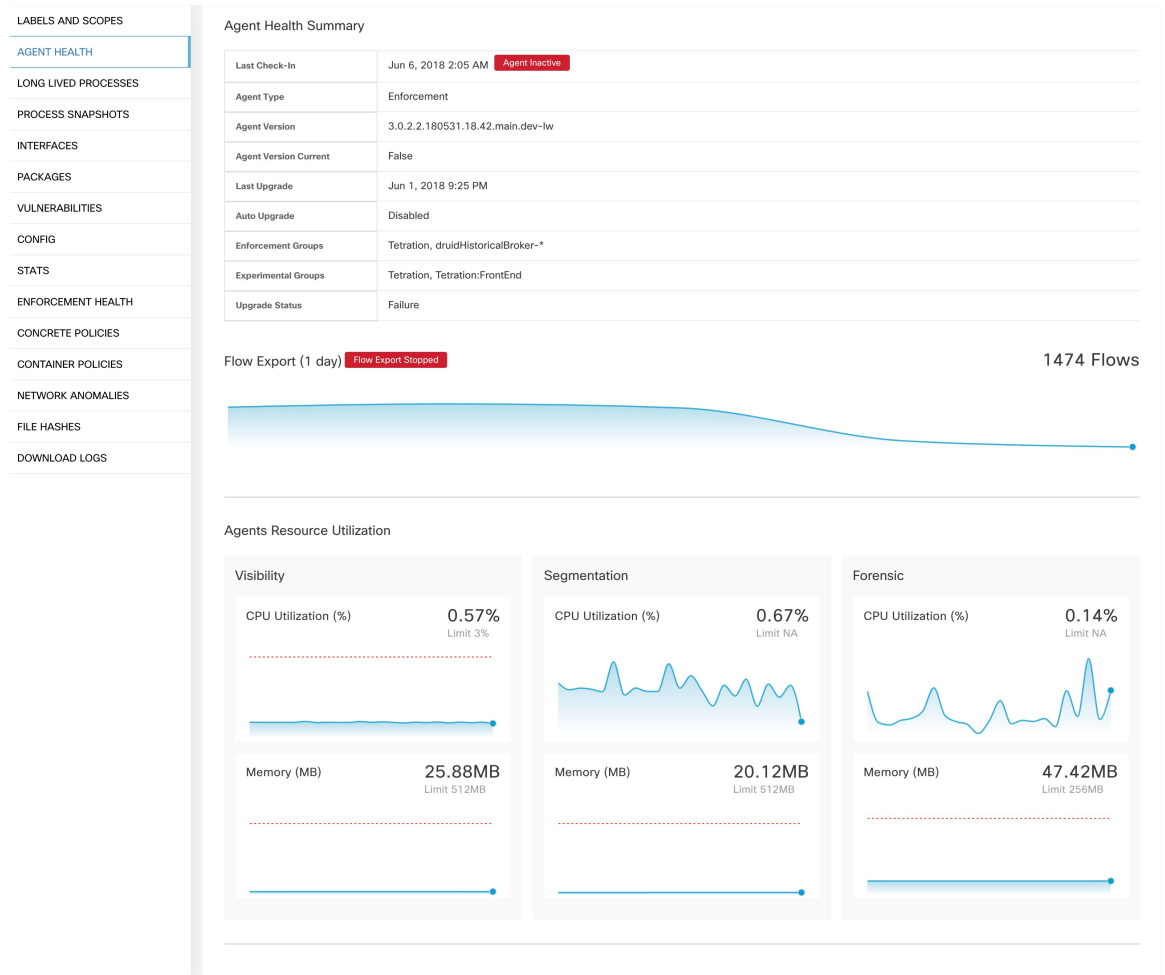
Figure 215: Workload Agent Health Details
