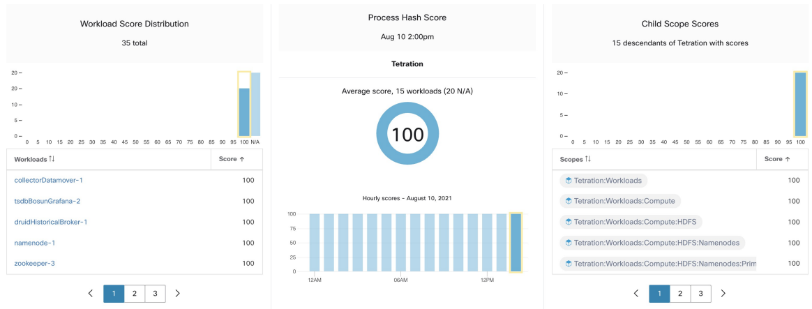
Figure 353: Process Hash Score Section in Security Dashboard
