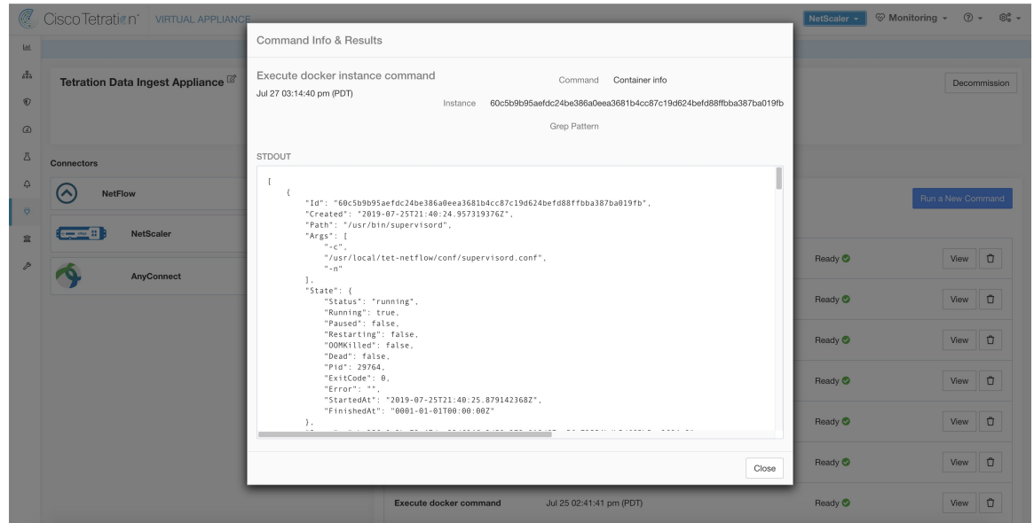
Figure 141: Execute a docker instance command on Secure Workload Ingest appliance to retrieve container info
