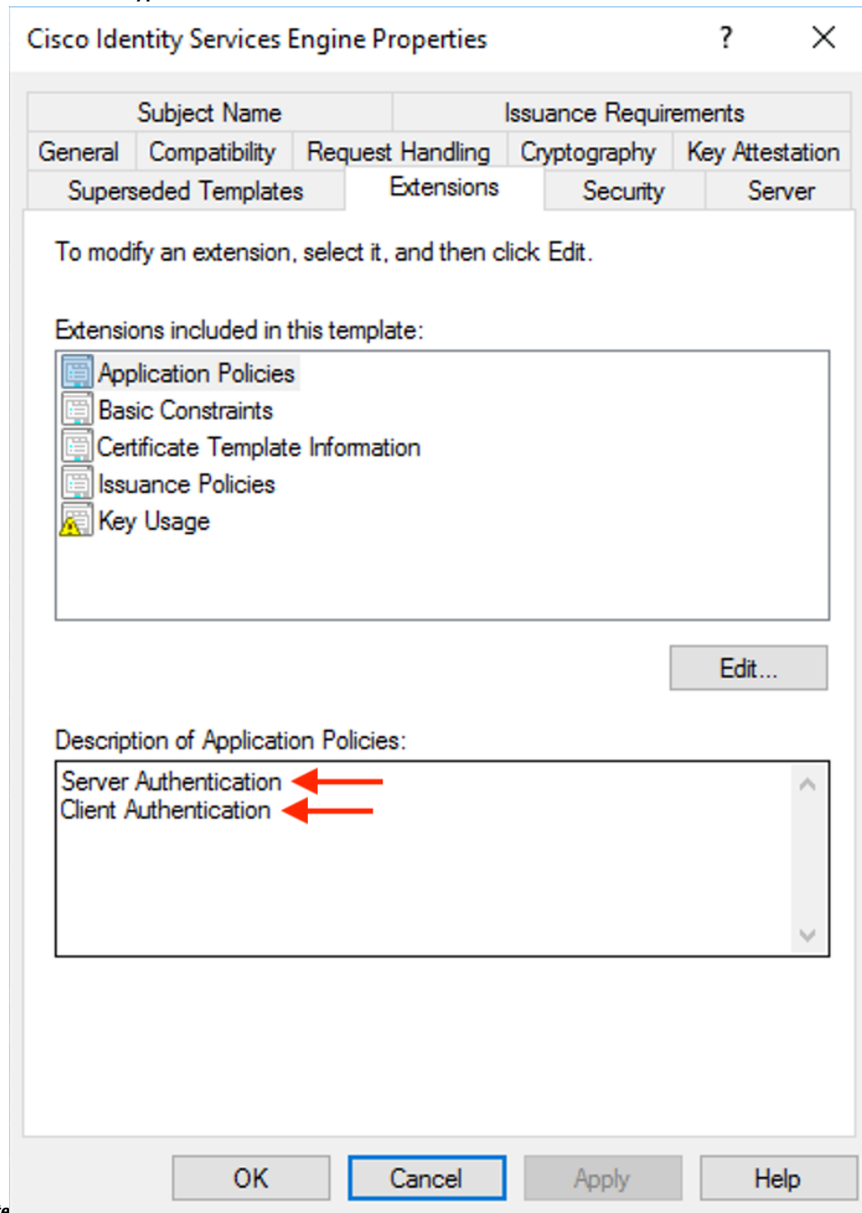
Figure 64: Extensions of Application Policies for a Certificate
