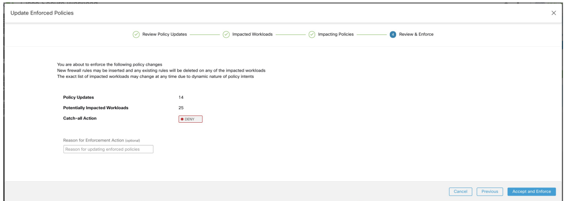
Figure 310: Review the Summary and Enforce Policy Changes
