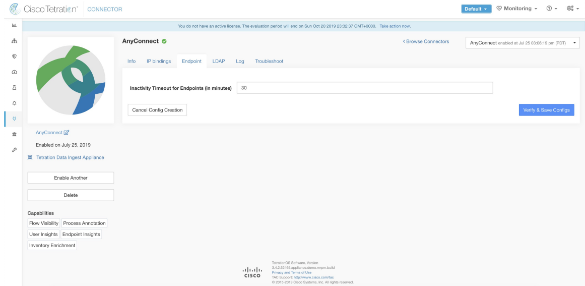
Figure 128: Endpoint inactivity timeout configuration on AnyConnect connector
