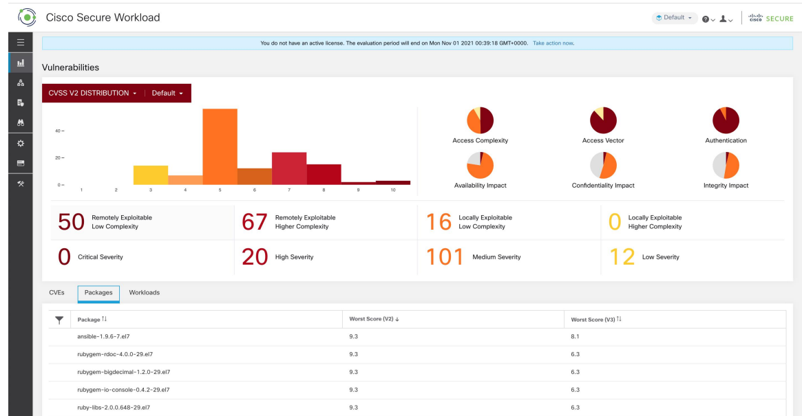
Figure 512: Packages Tab Listing Vulnerable Software in Specified Scope
