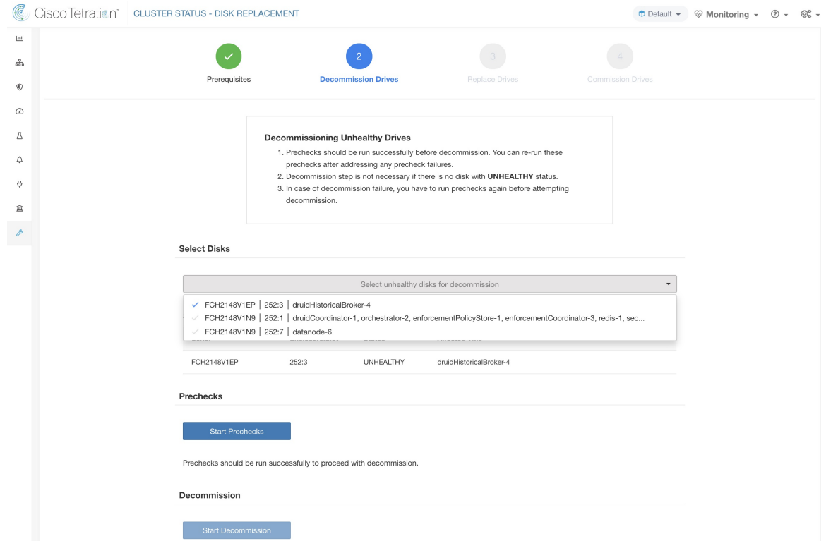
Figure 454: Unhealthy Disks for Decommission
