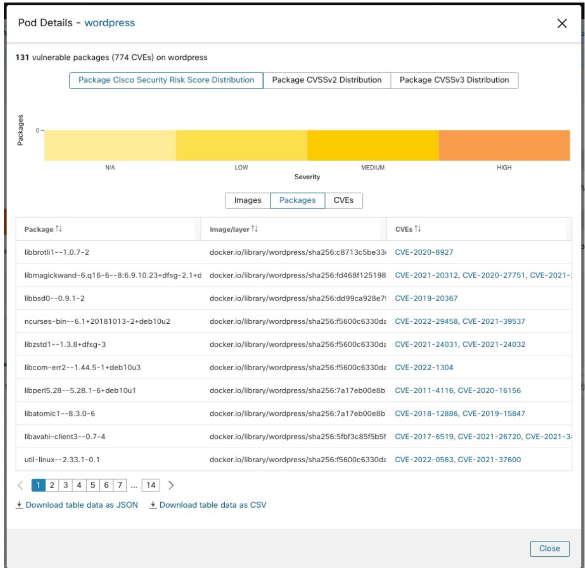
Figure 516: CVEs and Affected Packages in a Kubernetes Pod
