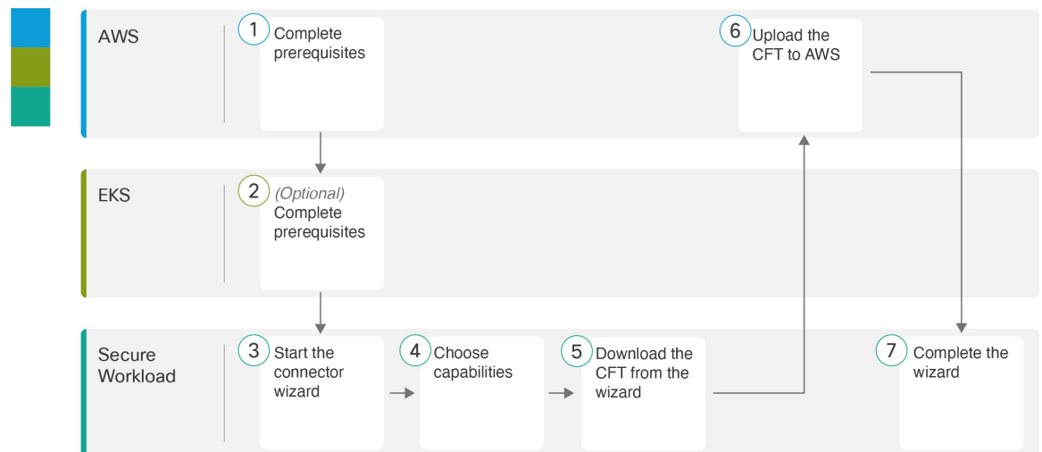
Figure 90: AWS connector configuration overview
