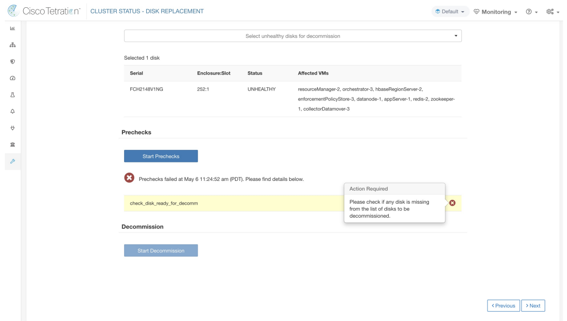
Figure 455: Suggested Action for Failed Precheck
