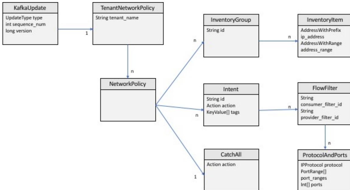
Figure 336: Data Model of Secure Workload Network Policy
