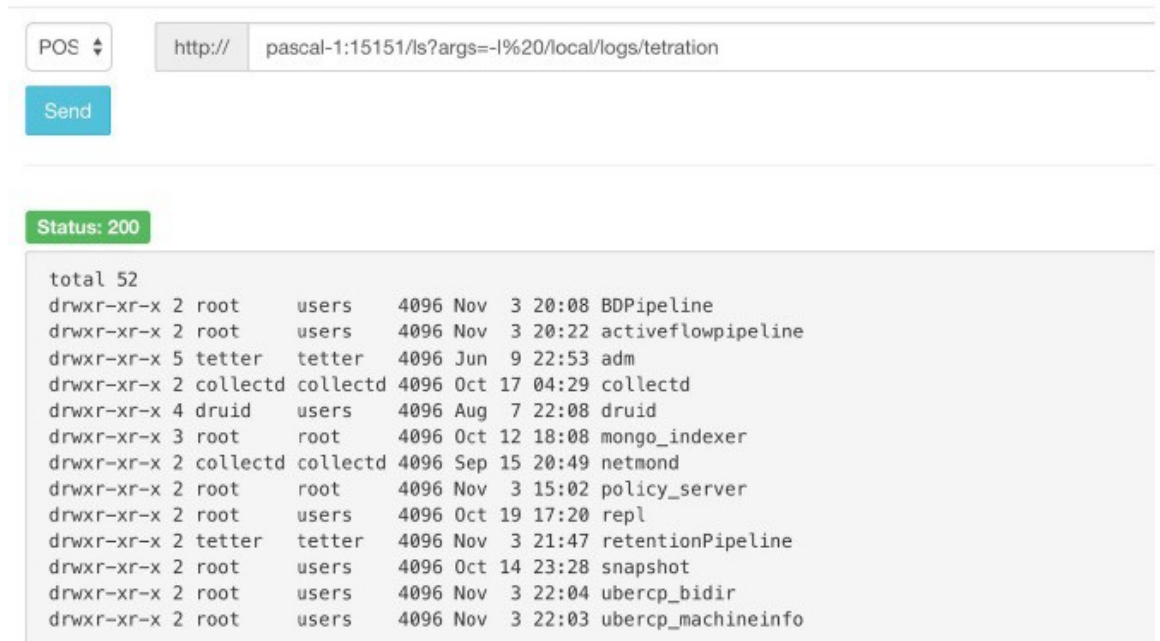
Figure 442: Using the Snapshot Service for Debugging and Maintenance
