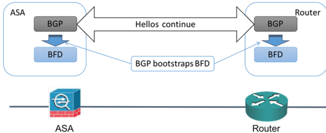
Figure 44: BFD Session Initiated
