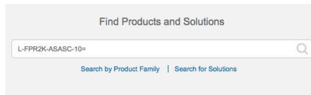
Figure 8: License Search
