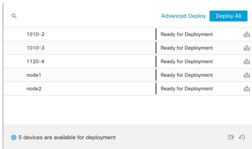
Figure 71: Advanced Deploy
