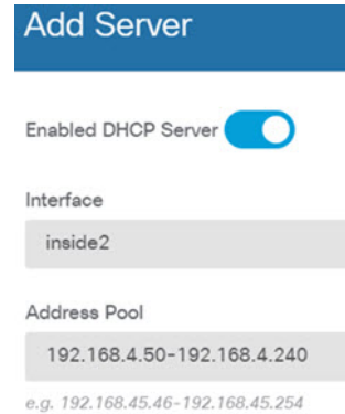
Figure 82: DHCP Server
