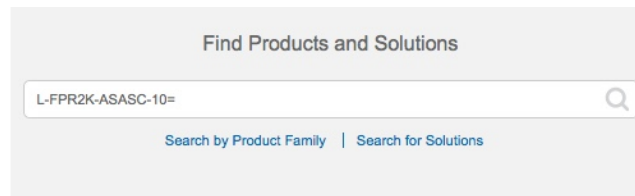
Figure 87: License Search
