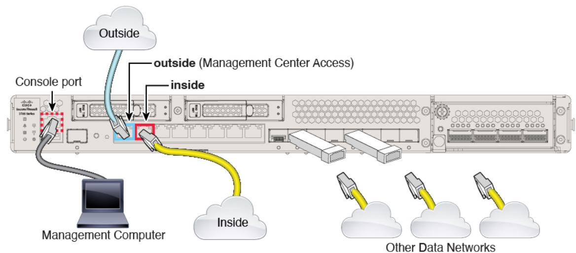
Figure 39: Cabling a Remote Management Deployment
