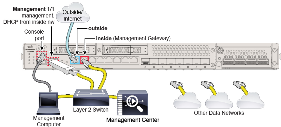
Figure 4: Cabling an Edge Deployment
