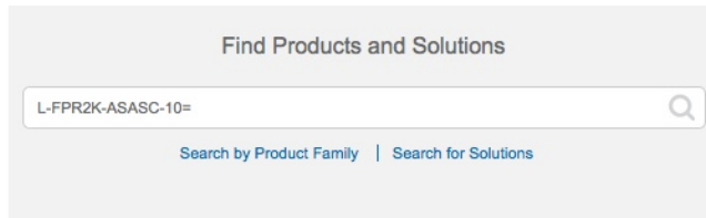
Figure 77: License Search
