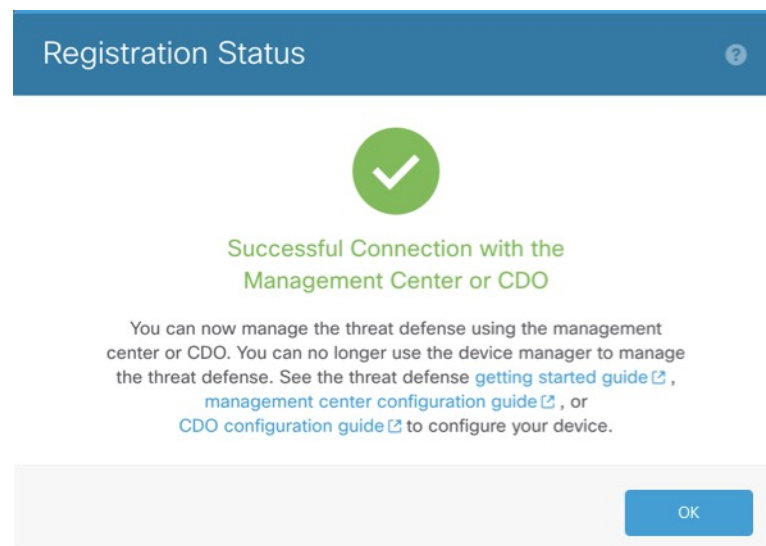
Figure 38: Successful Connection
