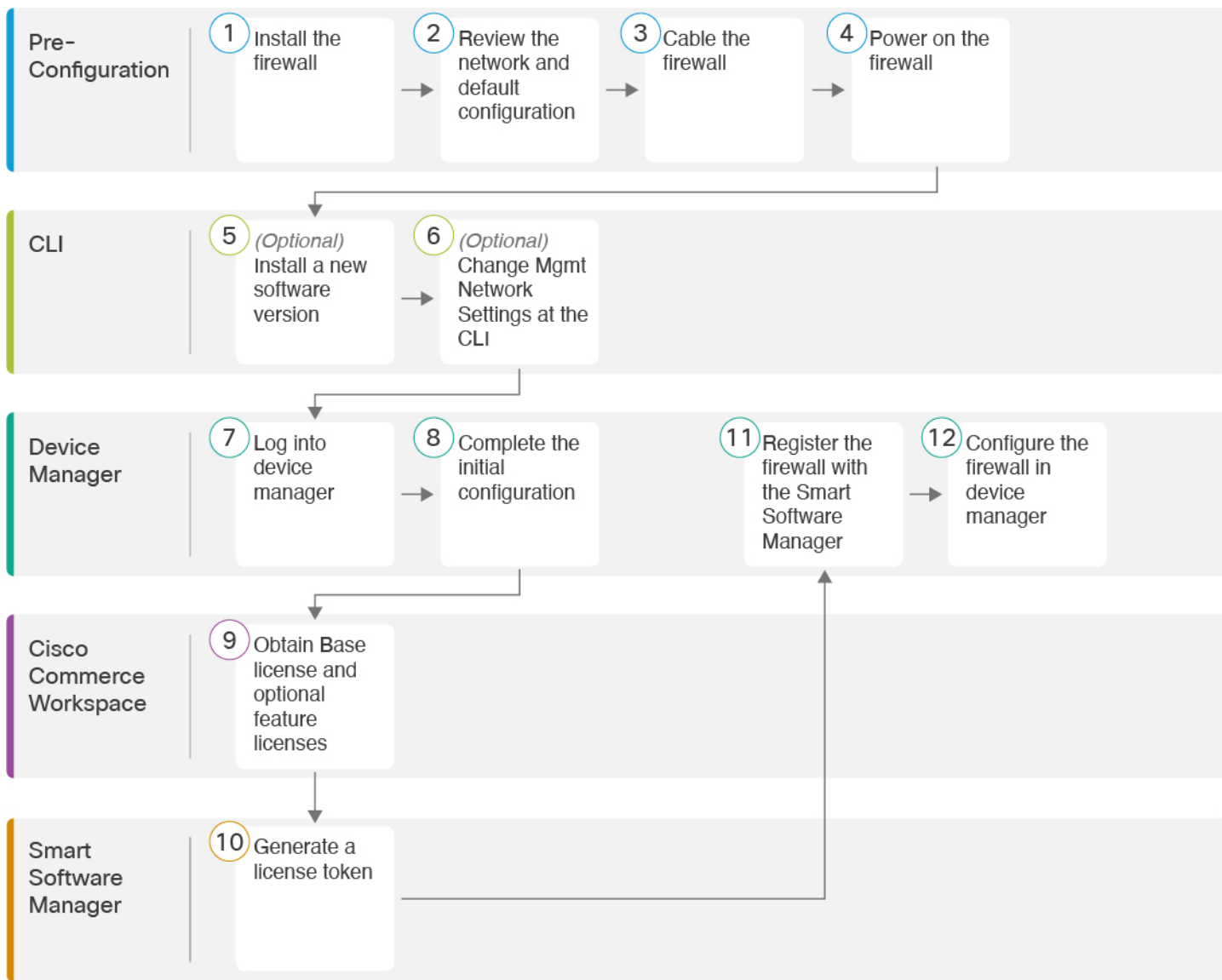
Figure 73: End-to-End Procedure
