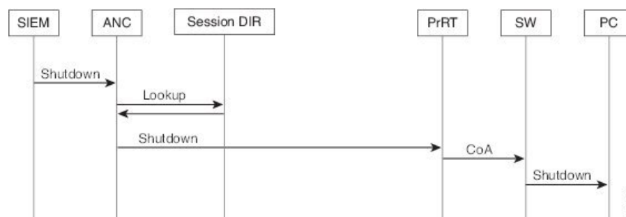
Figure 10: ANC Shutdown Flow
