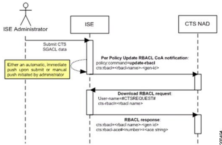
Figure 55: Update SGACL Content Flow
