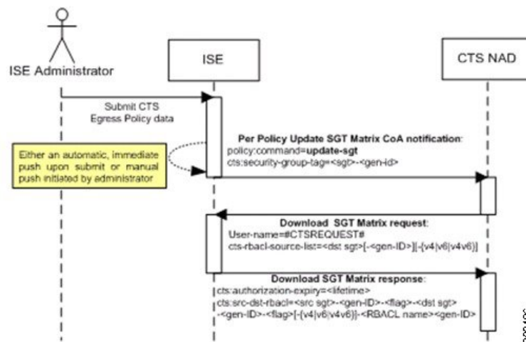
Figure 57: Update SGT Matrix CoA flow
