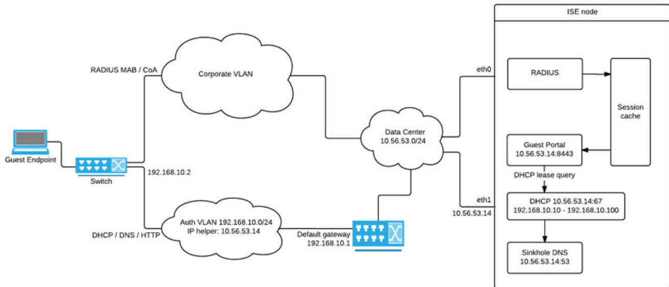
Figure 29: Auth VLAN Configured with IP Helper
