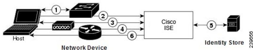
Figure 51: RADIUS-Based Authentication with EAP
