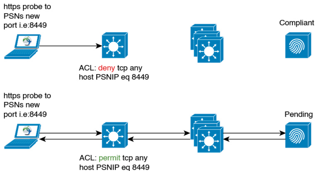
Figure 69: Posture State Synchronization
