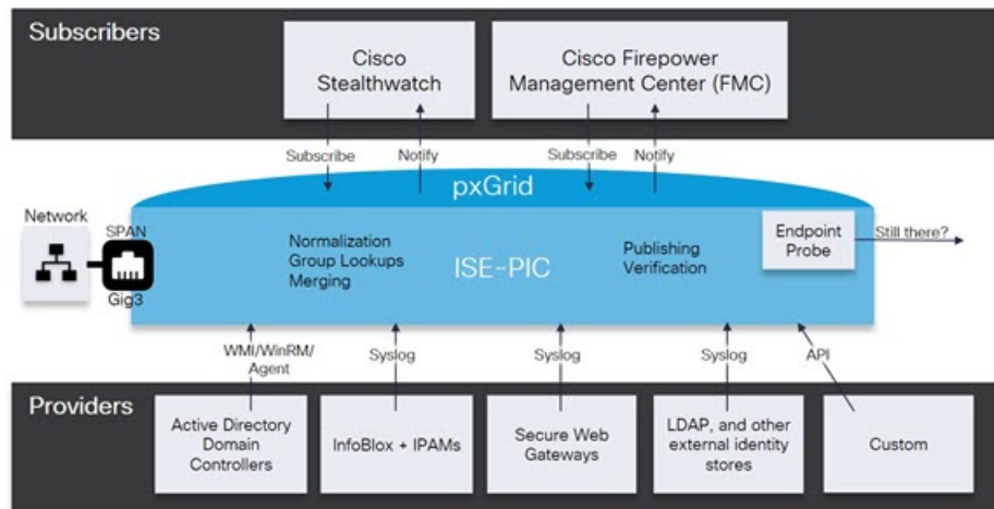
Figure 24: Passive Identity Service Flow
