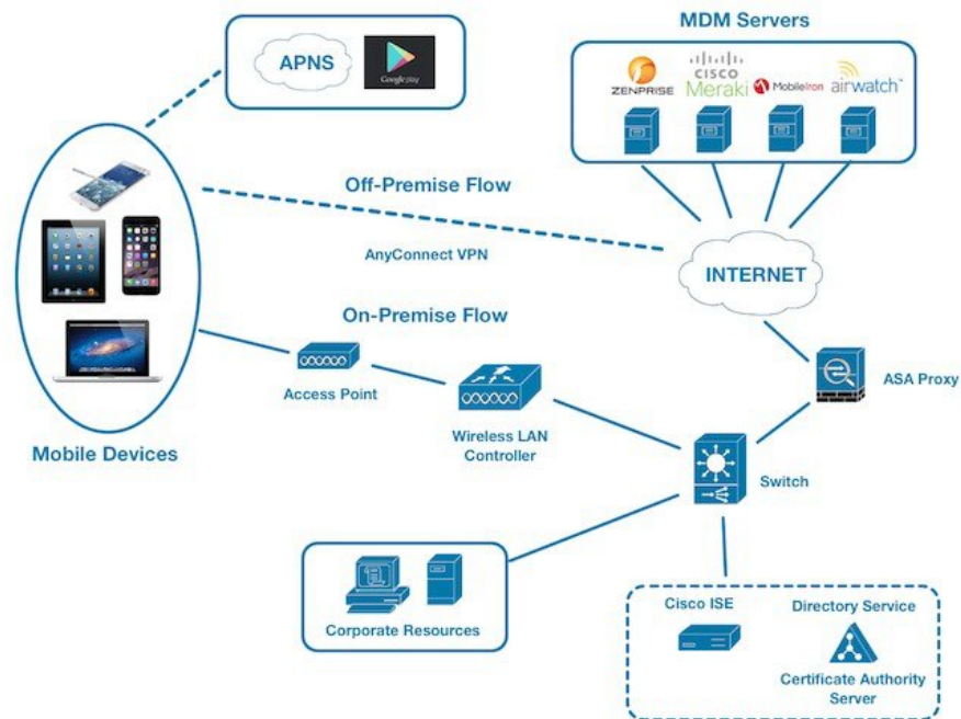
Figure 30: MDM Interoperability with Cisco ISE
