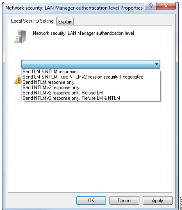
Figure 14: MS NTLM Authentication Type Options
