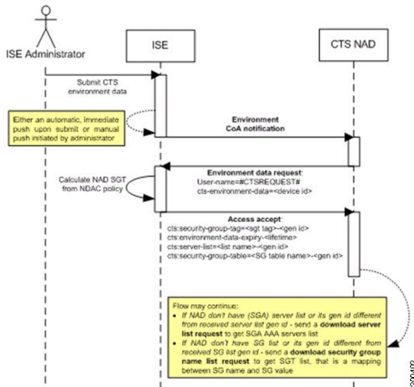
Figure 54: Environment CoA Notification Flow
