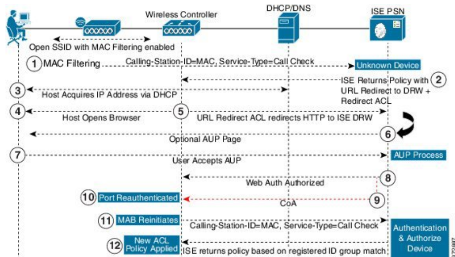
Figure 13: Wireless Device Registration Web Authentication Flow
