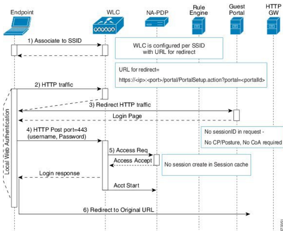
Figure 12: WLC with Local WebAuth Non-Posture Flow
