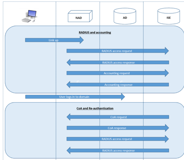
Figure 18: Easy Connect Enforcement Mode Detailed Flow
