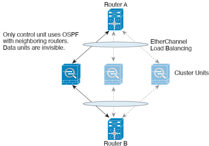
Figure 42: Dynamic Routing
