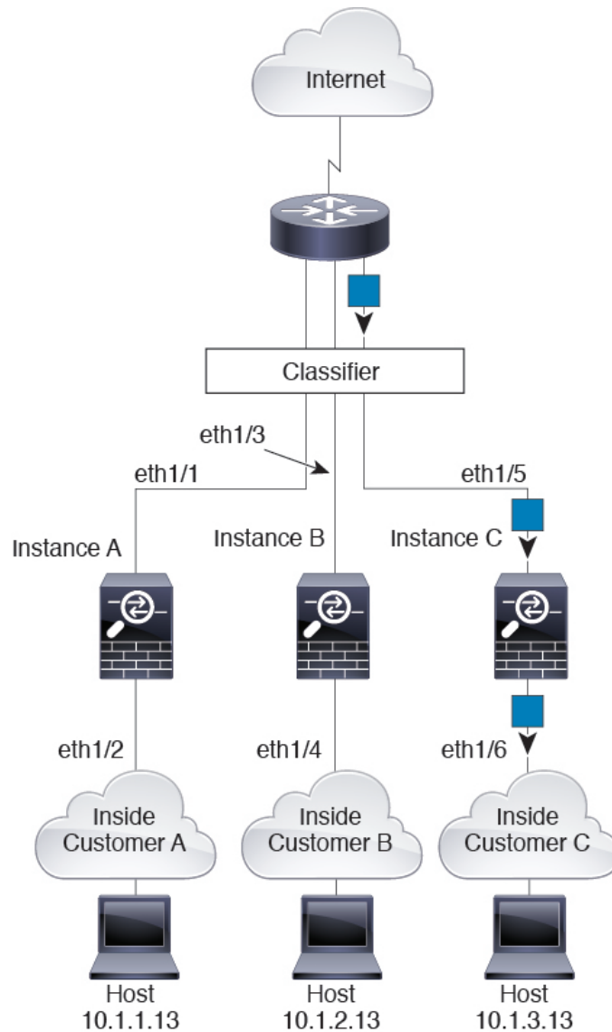
Figure 24: Inline Sets
