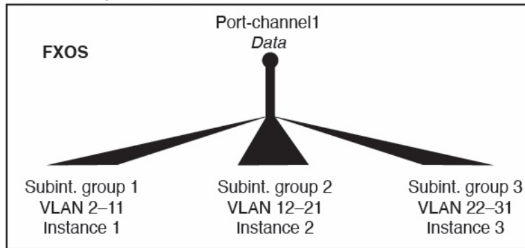
Figure 16: VLANs in FXOS vs. the Application for Container Instances
