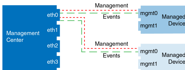
Figure 51: Single Management Interface on the Firepower Management Center
