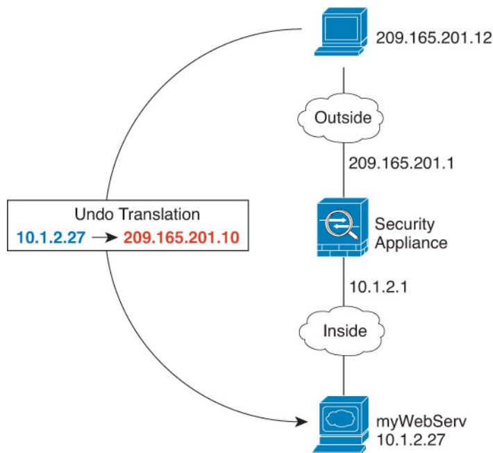
Figure 68: Static NAT for an Inside Web Server
