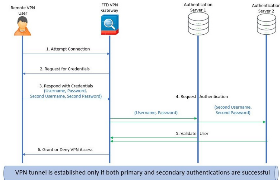
Figure 46: Remote Access VPN Secondary or Double Authentication
