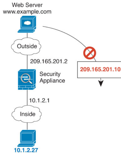
Figure 59: Remote Host Attempts to Initiate a Connection to a Mapped Address
