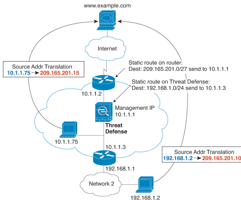
Figure 56: NAT Example: Transparent Mode
