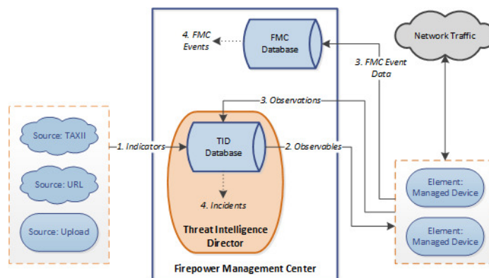
Figure 77: Firepower Management Center Data Flow
