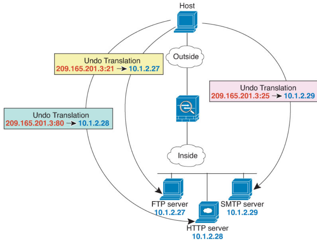
Figure 71: Static NAT-with-Port-Translation
