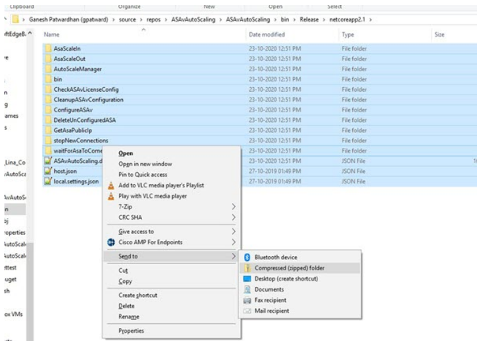
Figure 36: Build ASM_Function.zip
