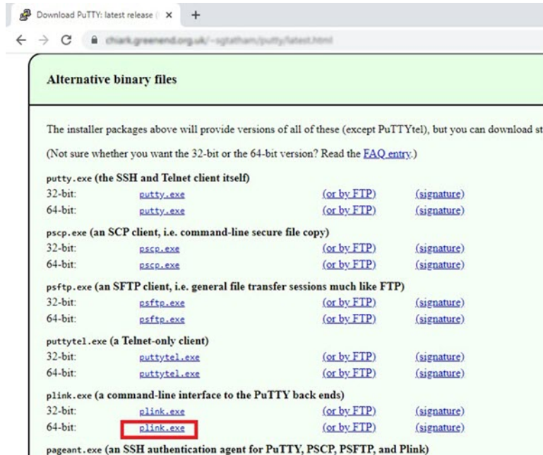
Figure 25: Download PuTTY
