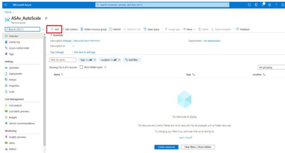
Figure 17: Azure Portal
