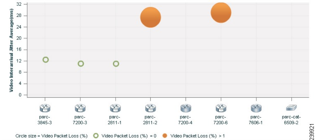
Figure 16: Video Interarrival Jitter and Packet Loss Graph
