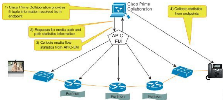
Figure 9: Interaction between Cisco Prime Collaboration Assurance and Cisco APIC-EM
