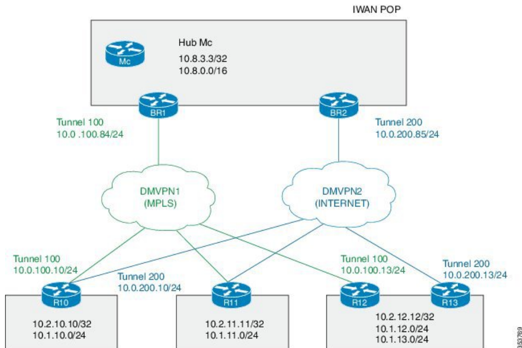
Figure 9: PfRv3 Topology
