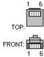
Figure 1: RJ12
