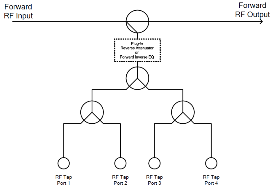
Figure 2. Block Diagram
