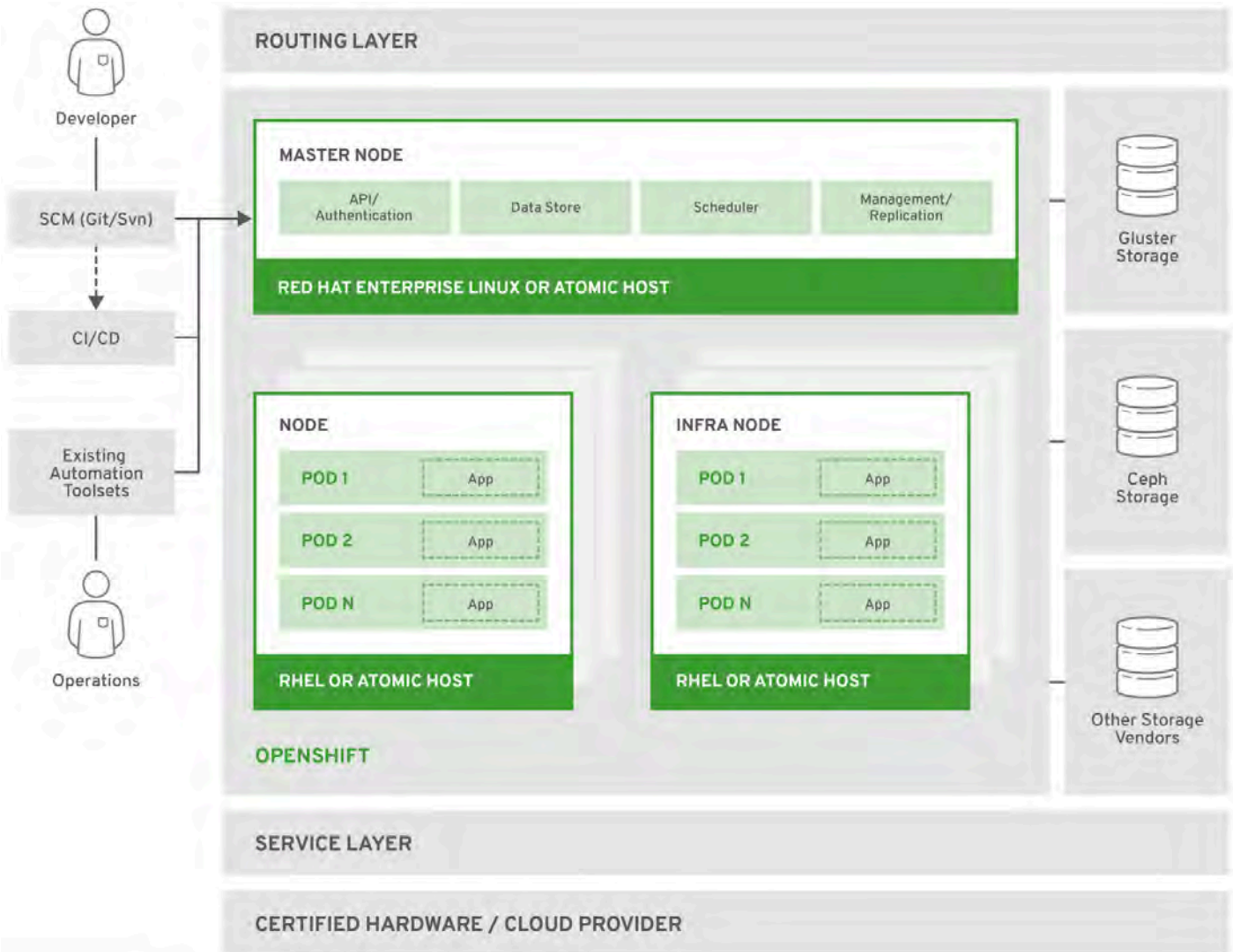
Figure 11. Architectural overview
