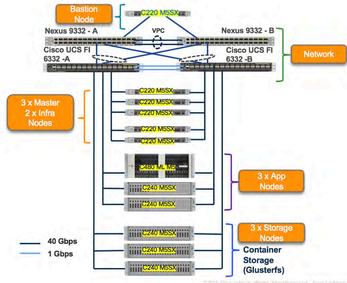
Figure 12. Red Hat OpenShift Container Platform architecture: Physical topology
