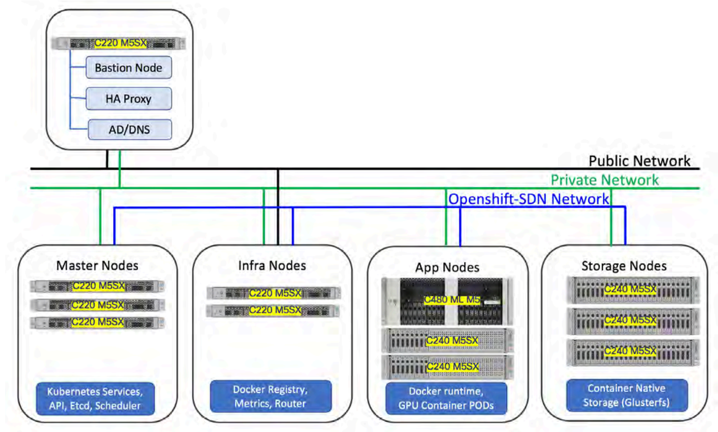
Figure 14. Network layout
