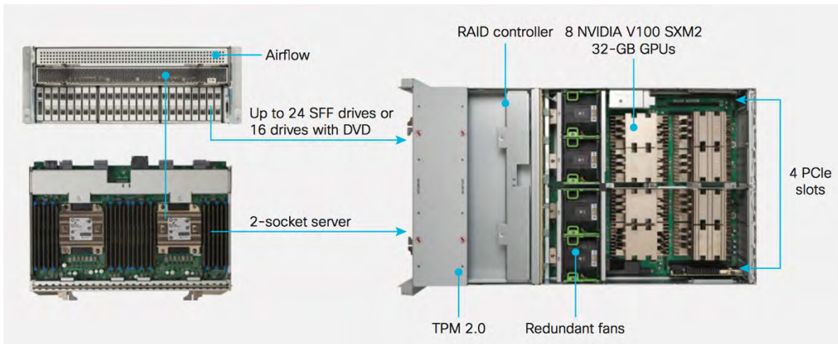
Figure 4. Cisco UCS C480 ML M5 Rack Server physical design
