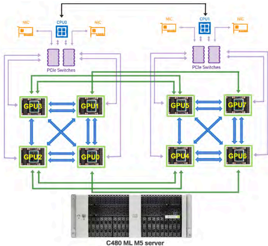
Figure 3. NVIDIA NVLink topology of UCS C480 ML M5
