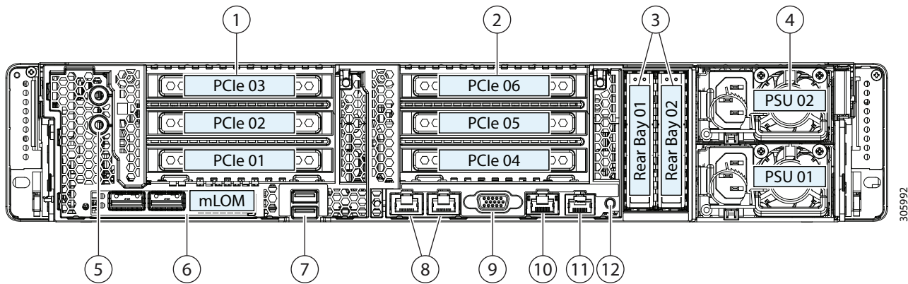
Figure 4 Chassis Rear View
