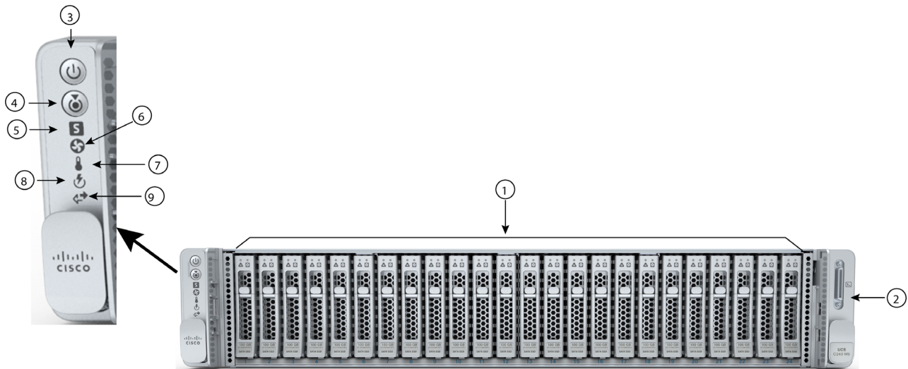
Figure 2 Chassis Front View: HXAF240C-M6SN (All NVMe)
