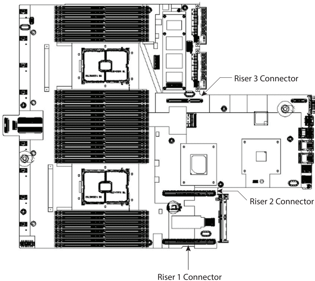
Figure 10 Cisco HyperFlex Express HX220C M6 All NVMe/All Flash/Hybrid Server Nodes Riser Connector Locations
