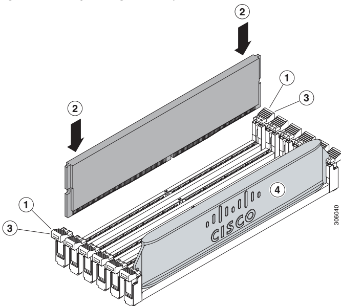
Figure 13 Replacing Memory
